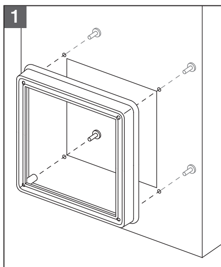
FPFA12 cut out
